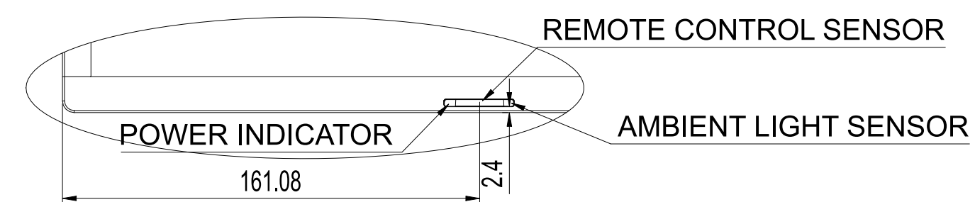
DETAIL C
