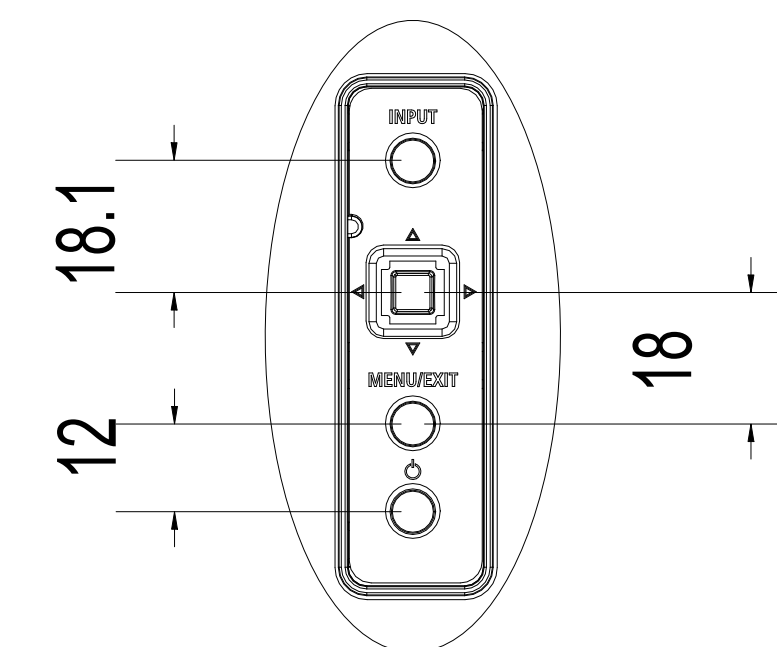
DETAIL D
