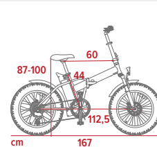
E-bike dimensions
